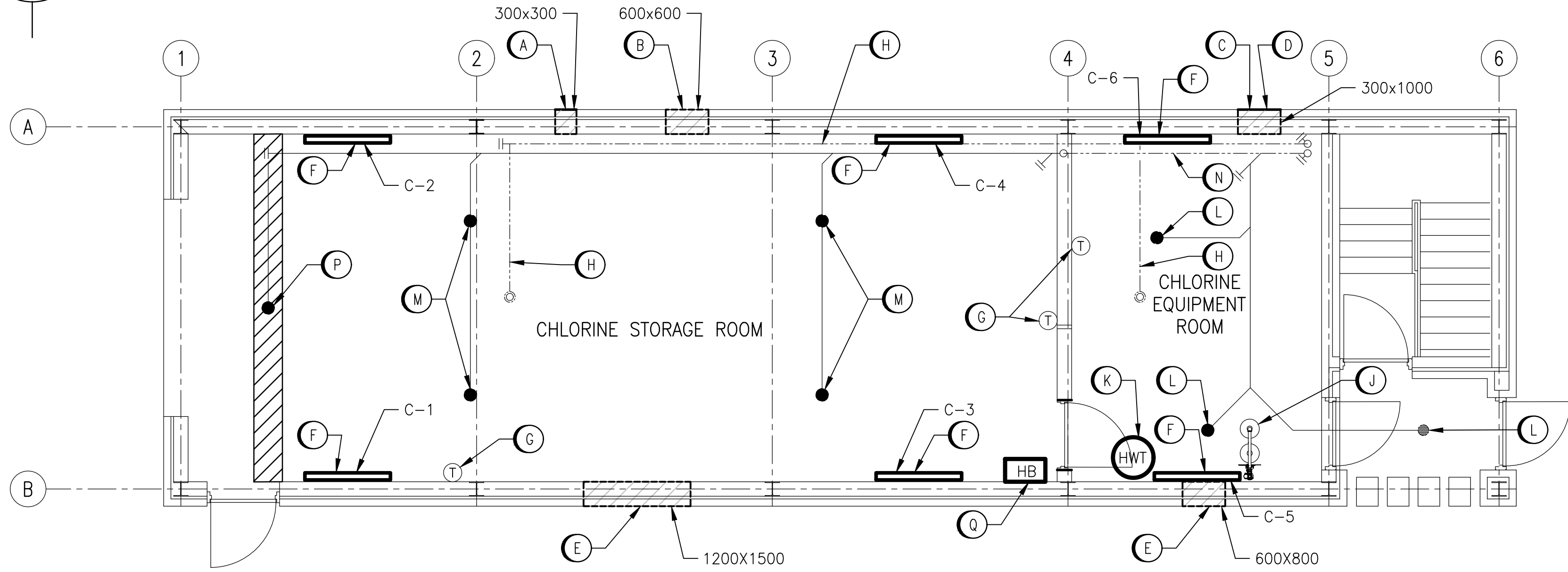
MAIN FLOOR PLAN SCALE: 1 : 50
